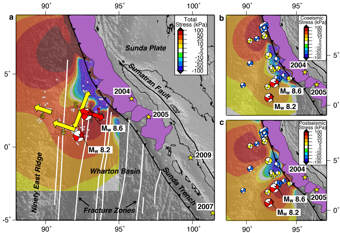
Figure 5.3: Recent stress changes in the Indian Ocean. (a) Total stresses induced by the 2004 [Chlieh et al., 2007], 2005 [Konca et al., 2007], and January M_w 7.2 [http://earthquake.usgs.gov/earthquakes/eqinthenews/2012/usc0007ir5/finite_fault.php] earthquakes, resolved at the 20 km hypocentral depth of the mainshock on the orientation of the initial WNW-ESE (red) fault plane [Meng et al., 2012]. Gray circles mark the first 12 days of the aftershock sequence (NEIC catalog). (b) Coseismic stresses induced by the 2004 and 2005 earthquakes. The yellow focal mechanisms highlight the strike-slip earthquakes during the first year following the 2004 earthquake and the blue focal mechanisms depict the remaining events before the 2012 mainshock (Global CMT catalog). (c) Cumulative postseismic stresses induced by the 2004 and 2005 earthquakes at the time of the 2012 mainshock.
