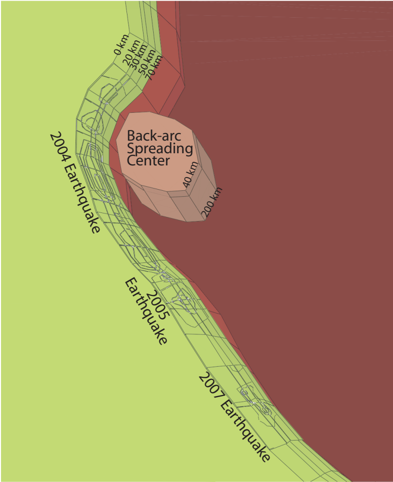
Figure 6.10: 3-D geometry used in the Back-arc Earth Model.
