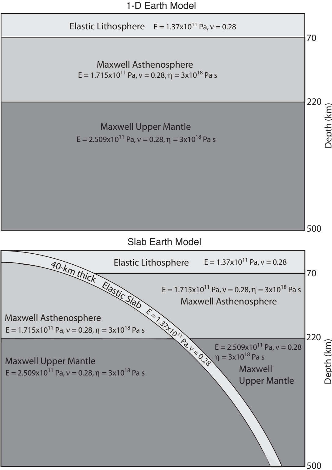
Figure 6.8: 1-D and Slab Earth Model schematics
