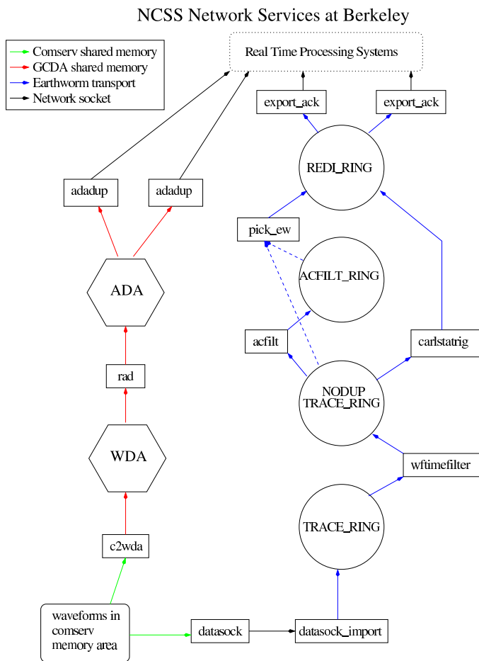
Figure 4.6.2: Flow of data from comserv/qmaserv areas through network services processing. One stream of the network services provides picks (and currently still provides codas) determined using the programs shown in the right flow path. Every five seconds, ground motion parameters are also determined, including PGA, PGV, PGD, and ML100 (left flow column). Parameters from the network services are available to the AQMS software for event detection and characterization. Data are also logged to disk (via datalog ), distributed to other computers ( mserv ), and spooled into a trace ring for export.
