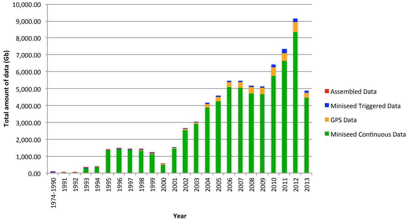
Figure 4.8.2: Figure showing the total volume of data archived at the NCEDC, broken down by data year.
