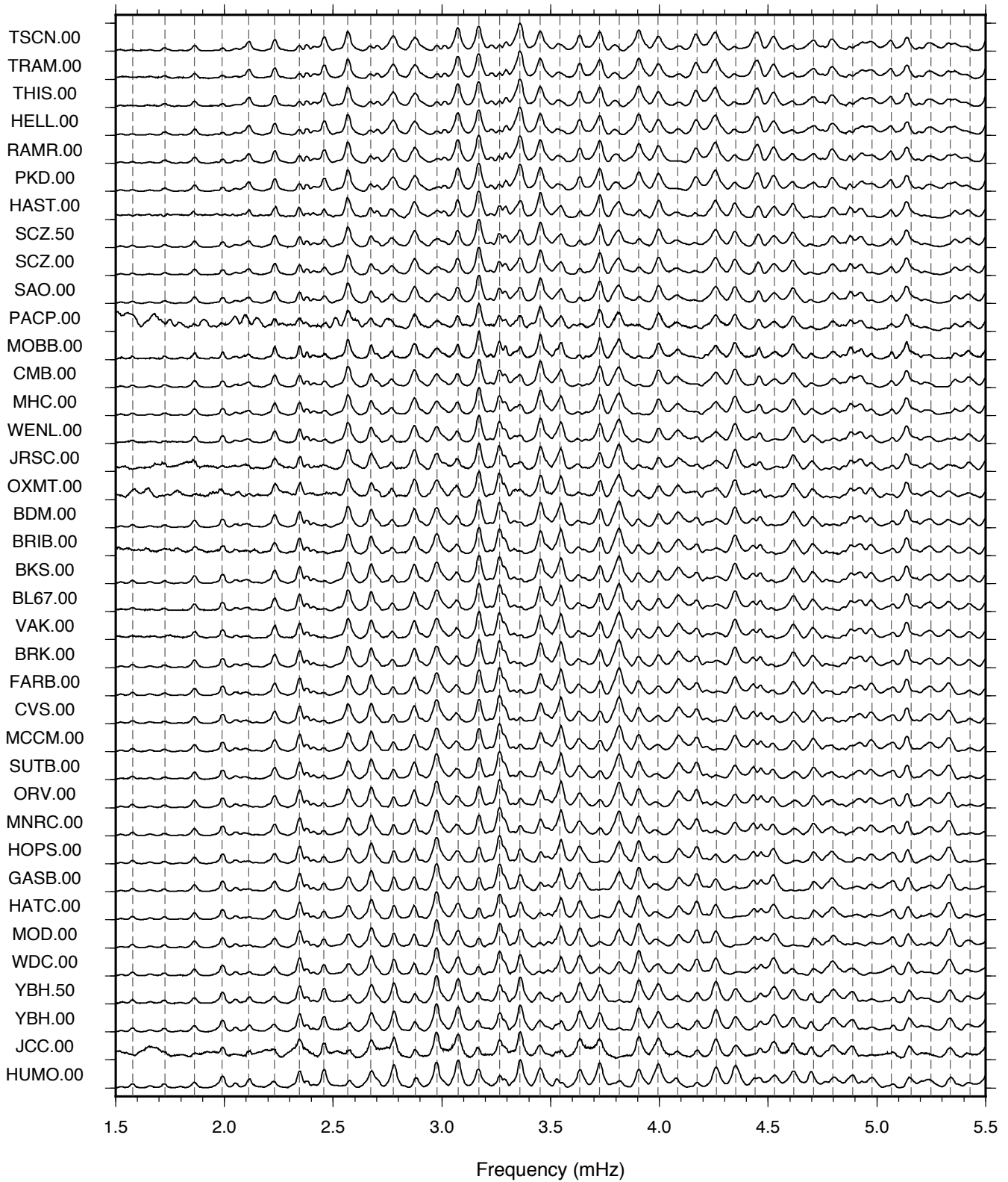
Figure 4.1.4: Amplitude spectra of vertical components of ground acceleration for the 120-hour-long data recorded at the BDSN stations following the May 24, 2013 M_w 8.3 Okhotsk teleseismic event. The spectra are normalized by their maximum amplitudes. Dashed lines are expected spheroidal modes with the PREM model.
