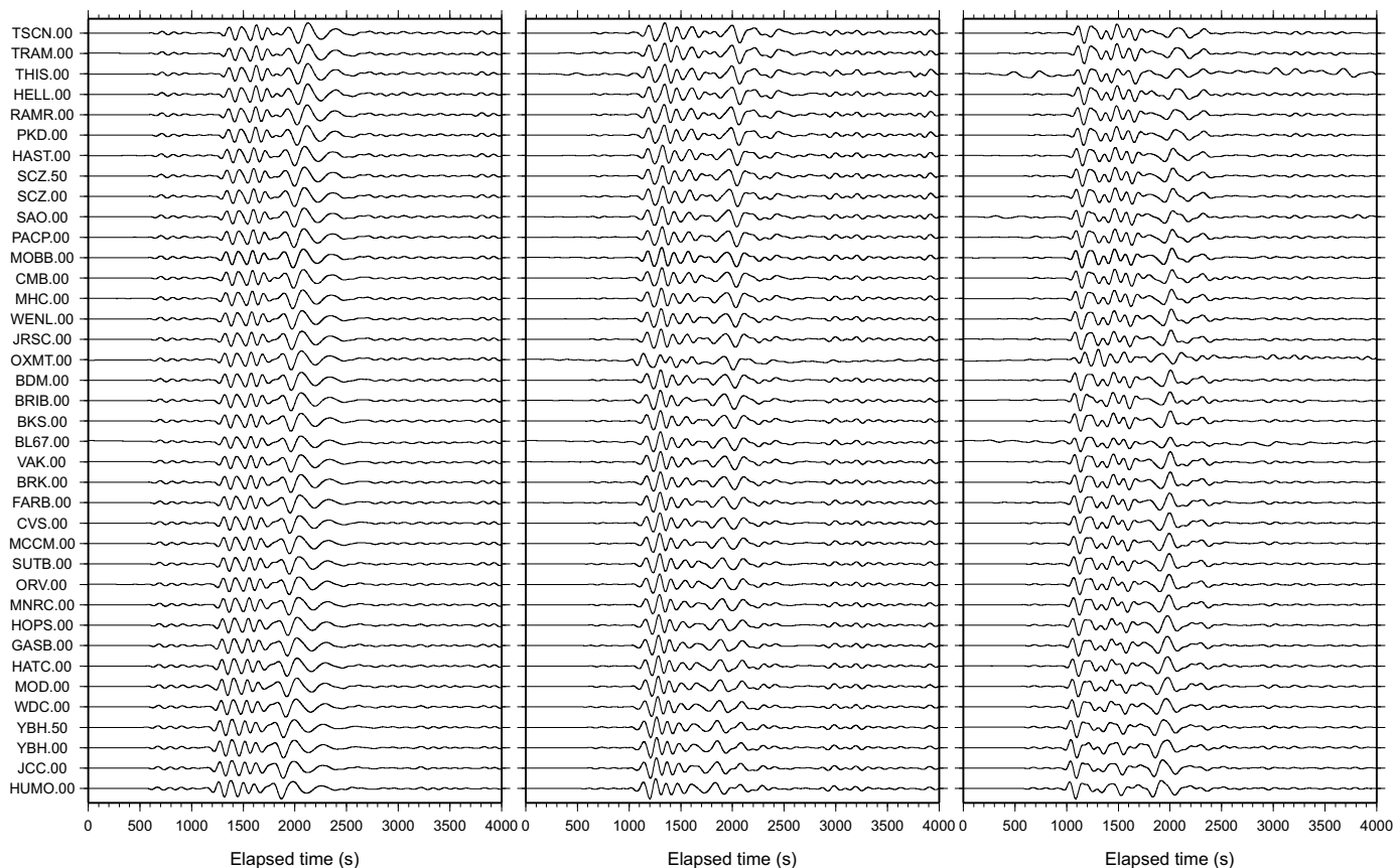
Figure 4.1.3: Long period (100-333 s period) waveforms recorded across BDSN from the M_w 8.3 teleseismic earthquake which occurred on May 24, 2013, Sea of Okhotsk at 54.874 N, 153.281 E. The panels show data from the vertical, north-south and east-west components, respectively. The traces are deconvolved to ground velocity, scaled by their maximum values, and ordered from bottom to top by distance from the epicenter. The highly similar waveforms recorded across the BDSN provide evidence that the broadband sensors are operating within their nominal specifications. The newest station, TCHL was installed in June 2013, after this earthquake occurred. BDSN data are archived and available at the Northern California Earthquake Data Center. This is described in detail in Operational Section 4.8.
