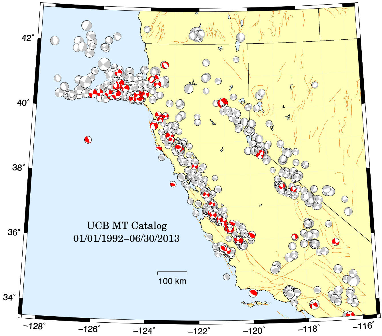
Figure 4.7.3: Map comparing reviewed moment tensor solutions determined by the BSL from past years (gray) with those from the fiscal year 2012-2013 (red/dark).
