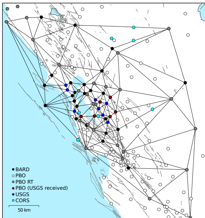
Figure 4.5.3: Map showing triangulated real-time processing network. Each black line represents an independent processing instance of trackRT.
