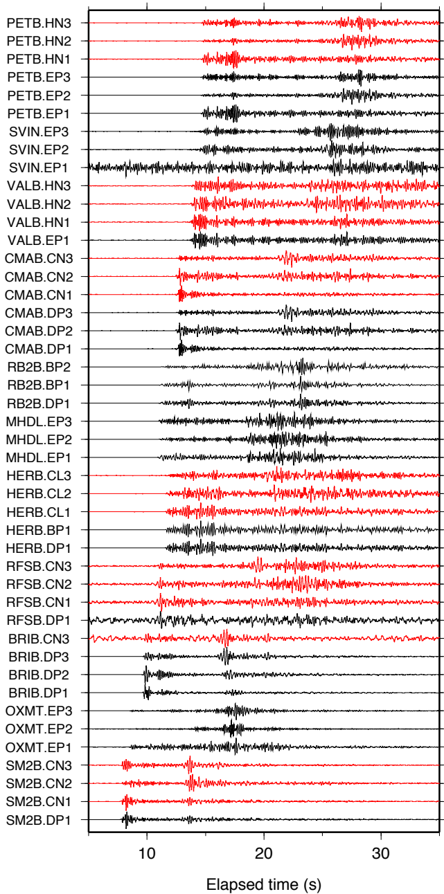
Figure 4.3.3: Plot of ground accelerations recorded on the geophones (black traces) and accelerometers (red/gray traces) of the 11 NHFN borehole stations in operation at the time of a recent Bay Area earthquake (February 24, 2013, M_{2.9} near Fremont, CA). The traces are filtered with a 1-8 Hz bandpass filter, scaled by their maximum values, and ordered from bottom to top by distance from the epicenter.
