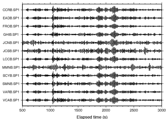
Figure 4.4.2: Plot of surface wave seismograms of the teleseismic M_w 8.3 deep earthquake in the Sea of Okhotsk (Lat.: 54.874N; Lon.: 153.281E; depth 609 km) occurring on May 24, 2013 05:44:49 (UTC) recorded on the SP1 (vertical) channels of the 12 HRSN borehole stations in operation at the time. Station RMNB no longer records data due to landowner issues. Here, vertical component geophone (velocity) data have been 0.05-0.10 Hz bandpass filtered and normalized by the maximum amplitude for each trace.
