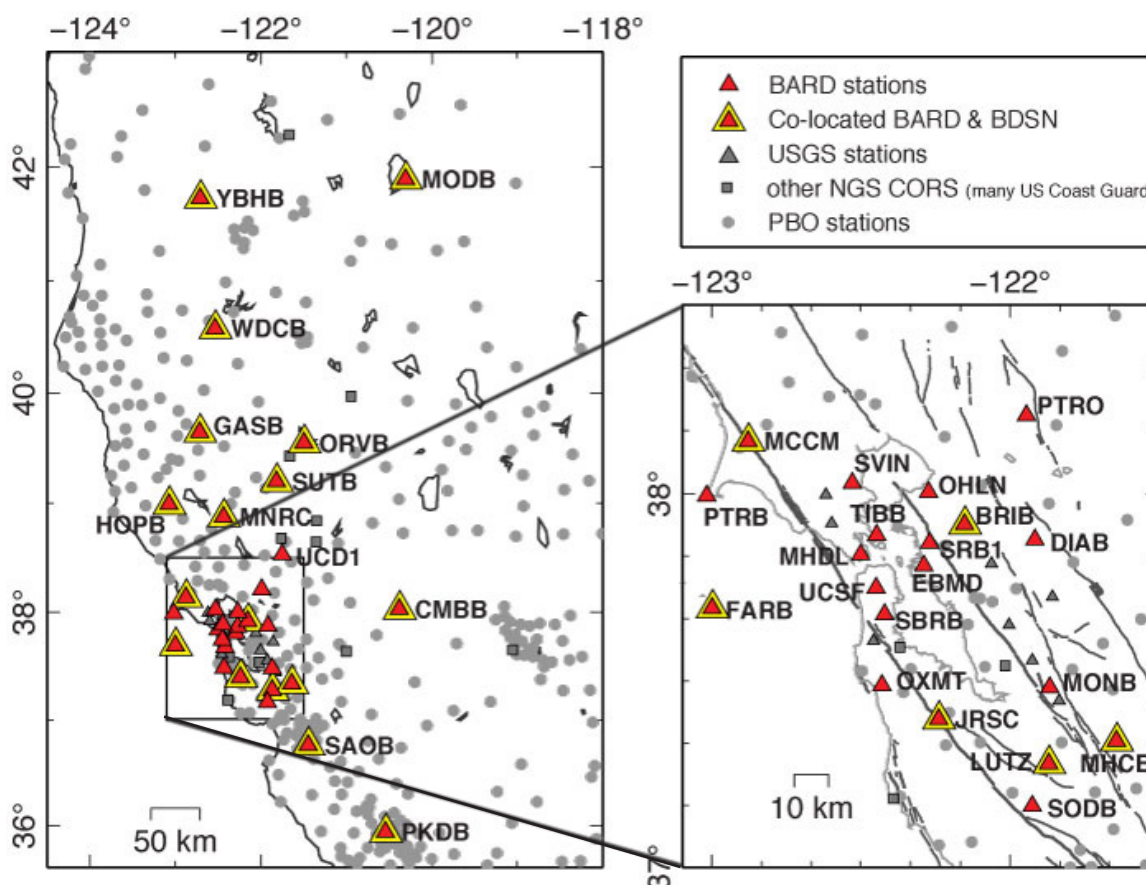
Figure 4.5.1: Map of the BARD Backbone network and surrounding PBO sites in Northern California. The right figure is an enlarged view of the box on the left figure.
