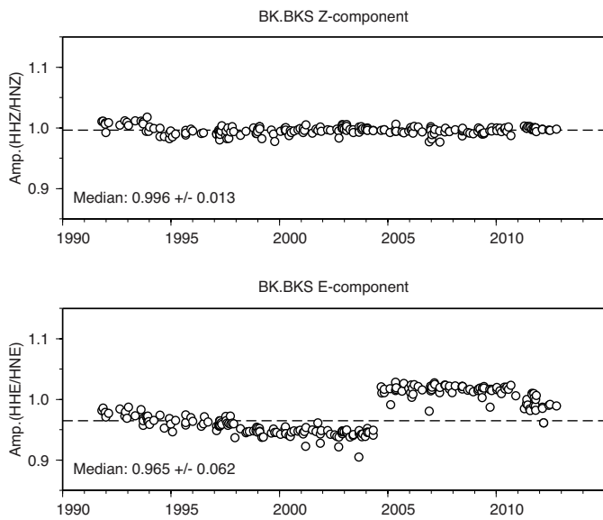
Figure 4.6.5: The temporal evolution of the amplitude ratio between the STS-1 broadband and strong-motion data at BK.BKS in the vertical and East-West components for a 20-year period. There were a number of upgrades of the equipment during this interval. The spectral amplitude ratio for the vertical component is stable over time, which indicates that the sensors' responses are stable and well described by the instrument response functions stored in the database. For the BKS East-West component, the median amplitude ratio has gradually decreased. This temporal reduction of the amplitude ratio is most likely due to a change in the characteristics of the STS-1E sensor induced by high humidity in the vault.
