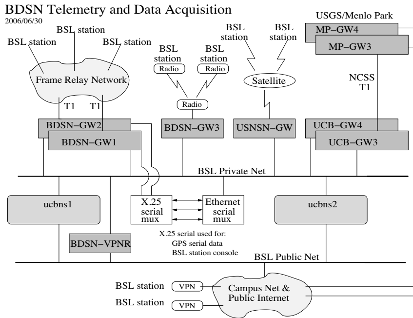
Figure 4.6.1: Data flow from the BDSN, NHFN, mPBO, HRSN, nad BARD networks into the BSL central processing facility.
