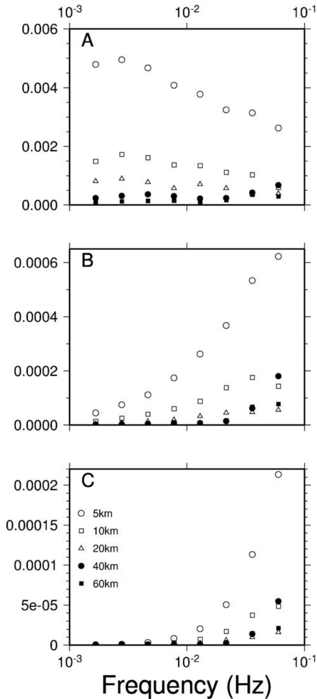
Figure 6. Peak time domain amplitude in (a) displacement, (b) velocity, and (c) acceleration in the first 3800 seconds of seismograms 5^\circ (137 km) from the source after narrow band filtering about central frequencies between 0.001 and 0.1 Hz for models with ice shell thicknesses ranging from 5 to 60 km.
