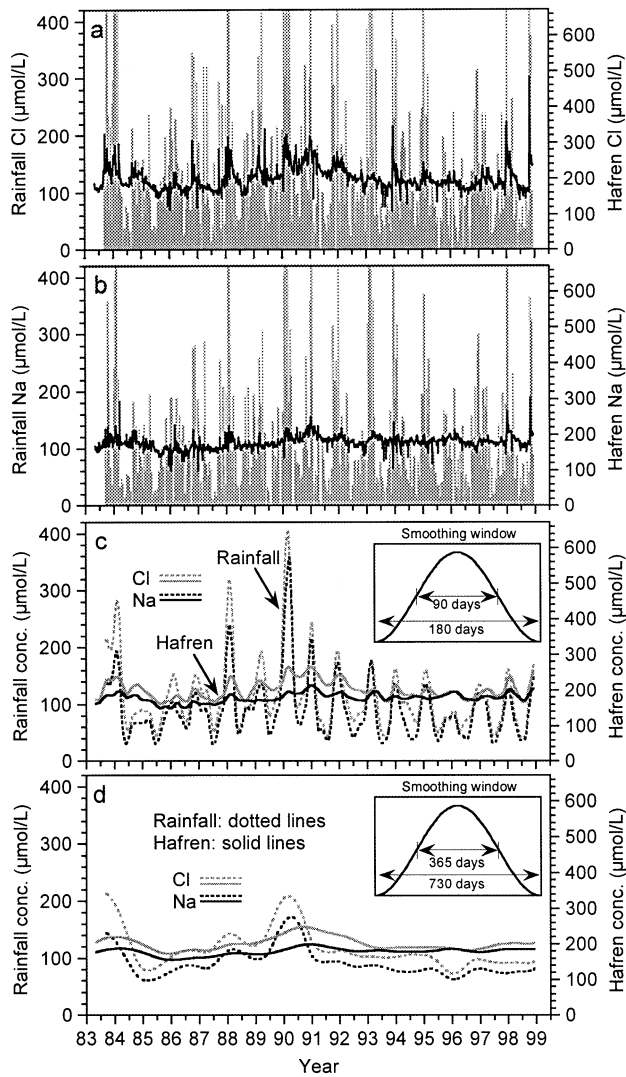
Fig. 2. Fifteen years of weekly measurements of sodium and chloride concentrations in rainfall and lower Hafren streamflow at Plynlimon, mid-Wales. Panels (a) and (b) show that concentrations in streamflow (black lines) are damped significantly compared to rainfall (grey lines). Panels (c) and (d) show ninety-day and annual moving averages of sodium (black) and chloride (grey) in rainfall (dotted lines) and streamflow (solid lines). Seasonal fluctuations in rainfall concentrations (dotted lines, panel c) vary greatly from year to year; seasonal fluctuations in streamflow concentrations (solid lines) are much smaller. The streamflow concentration scale has been expanded by a factor of 1.60, to account for dry deposition and evapoconcentration; that is, the weighted average concentrations of chloride in rainfall and streamflow would overlap exactly on the graphs. The sinusoidal smoothing windows (see insets) have a total width that is twice their nominal size (90 and 365 days in panels (c) and (d) respectively), which is their width at half maximum.
