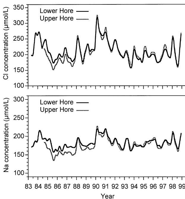
Fig. 5. Ninety-day moving averages of chloride (top panel) and sodium (bottom panel) in streamflow at lower Hore (black lines) and upper Hore (grey lines). The chloride concentration scale has been compressed by the sea-salt sodium/chloride ratio (0.86) to make the two scales comparable.
