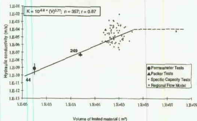
Figure 4. Relationship of hydraulic conductivity to scale of measurement in the Sinnipee Group of northeastern Illinois and southern Wisconsin. Permeameter and packer tests were plotted as geometric means with 95% confidence intervals; specific capacity tests and modeling values as single values. Notice the large scale packer test within the cloud of the specific capacity tests. Specific capacity tests were derived from two different sources and geographical areas. Number of observations are given adjacent to means. The regression line is derived from all individual values ( n = 357 ) below the model scale. The 95% confidence interval about the slope is 0.77 \pm 0.05 , and r is the correlation coefficient.
