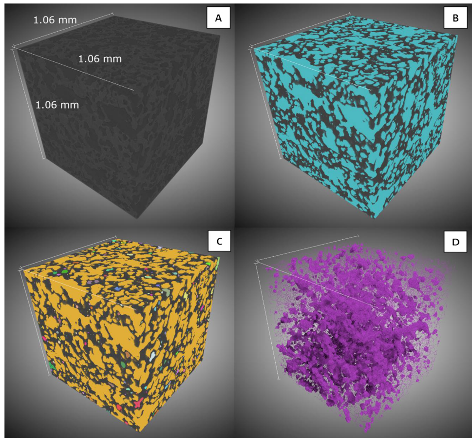
Fig. 3 3D visualization of L4. All three volumes have the same size and correspond to one VOI. (A) 3D reconstruction of L4. Darker voxels correspond to vesicles and the brighter ones correspond to the solid phase (B) Segmentation of the porous media represented in cyan color. (C) Separation of the vesicle phase. Every color represents a single bubble. (D) 3D visualization of the skeletonization of sample L4. The convoluted shape and the chaotic distribution of the purple matrix structure make it difficult to calculate classically defined tortuosity
