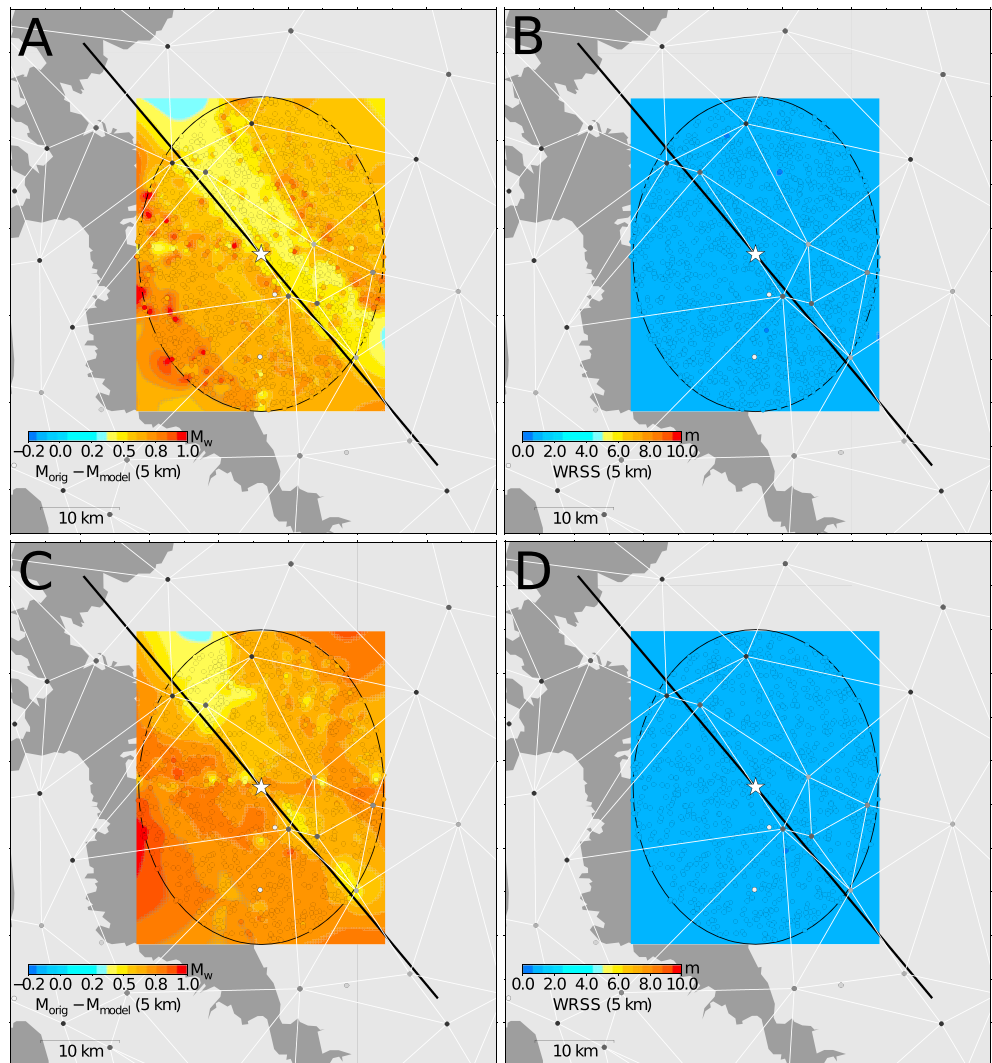
Figure 12. Same as Figure 11 except that the fault in the forward model ruptures from 5 to 12 km depth (inversion assumes surface rupture). Magnitude error increases and misfit field homogenizes even more compared to Figure 11.
