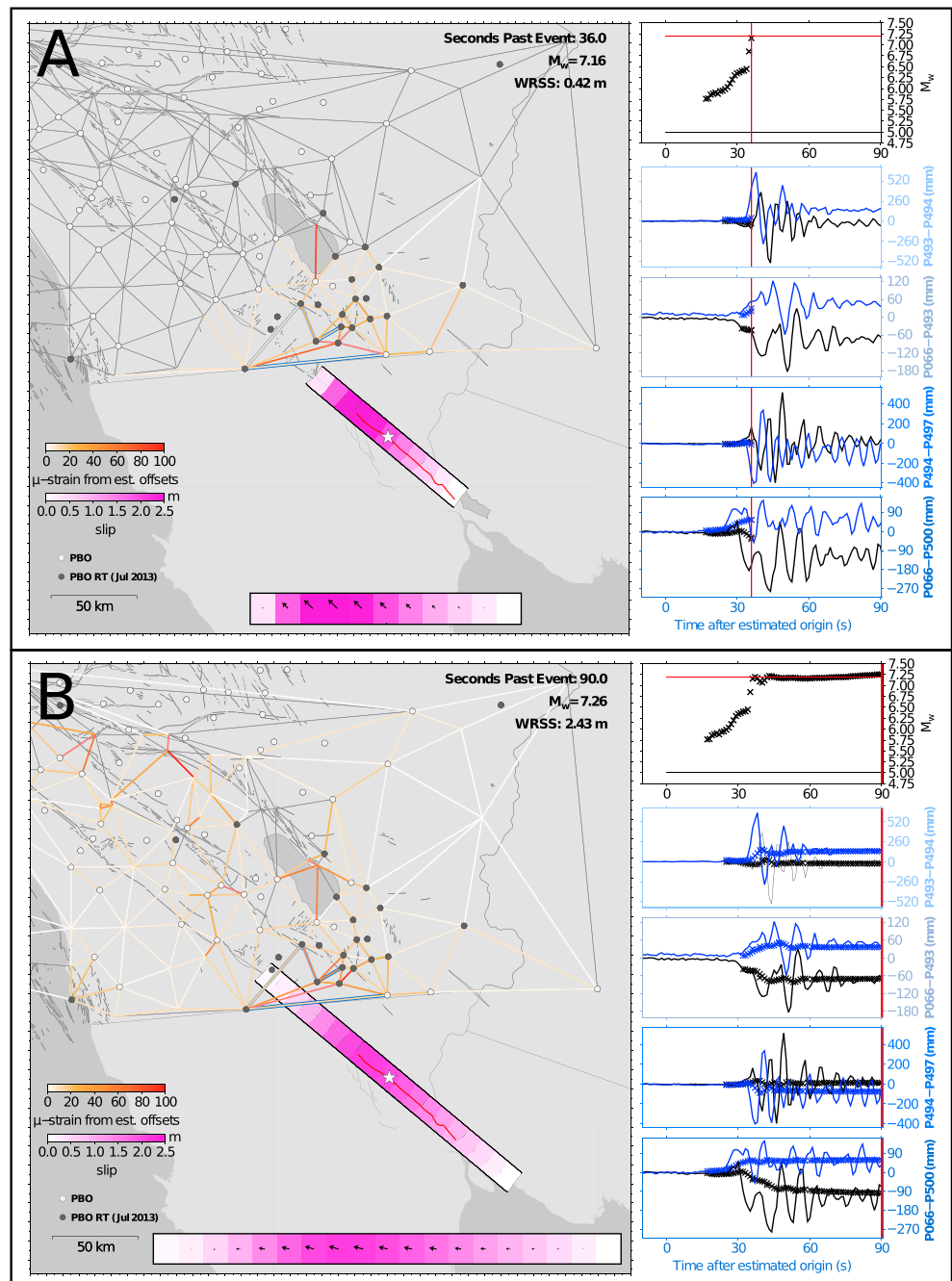
Figure 7. (a) Initial recovered slip model for El Mayor-Cucapah, 36 s after official event onset time. Similar to Figure 4, but color of baselines indicates microstrain along the respective baselines. Offset estimation (blue and black crosses in time series panels) begins too early due to strike slip rupture not starting until 15 s after event origin [Wei et al., 2011]; hence the early and low initial magnitude estimates. This snap shot shows a M_w = 7.16 solution 2 s after Colombelli et al. [2013] indicate static offset arrival and give their first solution at M_w = 7.08 . (b) Final recovered slip model and estimated offsets 90 s after event onset (see supporting information for full animation). Offset time series now clearly show the small impact of dynamic motion on offset estimation and hence magnitude estimation.
