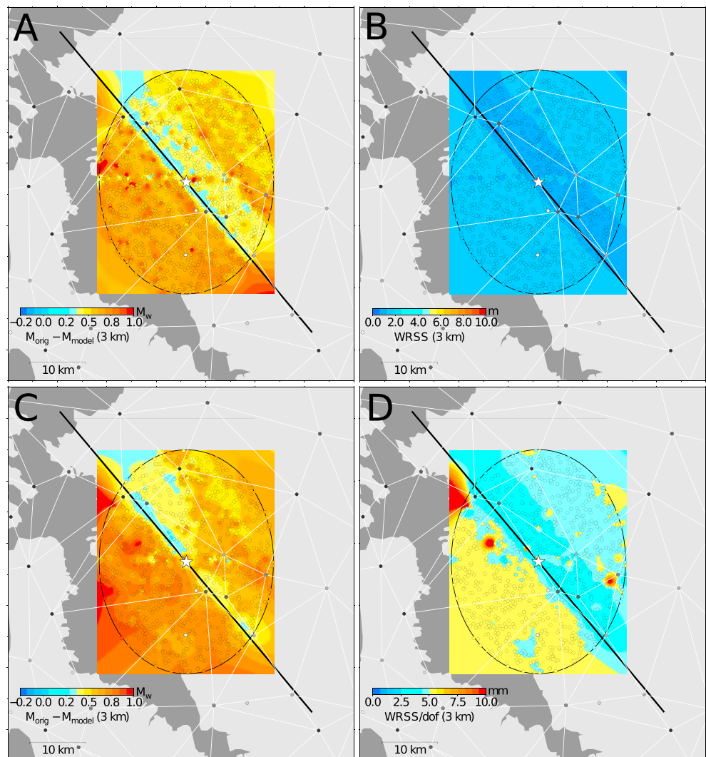
Figure 11. Same as Figure 10 except that the fault in the forward model ruptures from 3 to 12 km depth (inversion assumes surface rupture). Magnitude recovery is significantly decreased at generally good model fit. This is due to minimal or unphysical slip (with less Laplacian smoothing) being put in the model fault in the inversion.
