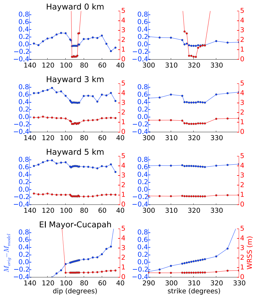
Figure 14. Sensitivities to a priori assumptions about strike and dip in the inversion. Three forward models (fault from 0, 3, and 5 km to 12 km depth, respectively) with 90 dip creating M_w 7.0 equivalent slip and the data from the El Mayor-Cucapah event are inverted multiple times. Each time we vary dip (left column) and strike (right column) of fault plane for the inversion. All panels show in blue the final error in magnitude recovery after the inversion ( \approx 4 min after event origin), while the red graphs show the respective WRSS misfit between input data and recovered model. The left column displays changes in dip which we varied from 45 to 135° for all cases (note that the plots order degrees of dip in decreasing order as this translates more intuitively to map view: 135–91° dip to the SW and 89–45° dip to NE). The right column shows changes in strike, which we varied from 290 to 330° for El Mayor-Cucapah and 300 to 340° for the synthetic Hayward cases. For all tests we increased the angles in 5° steps but decreased this interval to 1° steps around the nominally correct values. The dots in the panels mark the discrete test values. We connect the dots to guide the reader’s eye.
