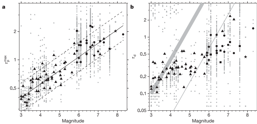
Figure 3 | The relation between \tau_p^{\max} , \tau_d and magnitude. a , The scaling relation between \tau_p^{\max} and magnitude for earthquakes in southern California (triangles), Japan (circles), Taiwan (squares) and Alaska (stars). Observations at individual stations can show a large scatter for a given event (small grey shapes). The event averaged values are also shown (large black shapes). The best-fit to event averages is shown as a solid line. The average absolute deviation of the observations is 0.54 magnitude units; plus and minus two times the average absolute deviation is shown as dashed lines.
