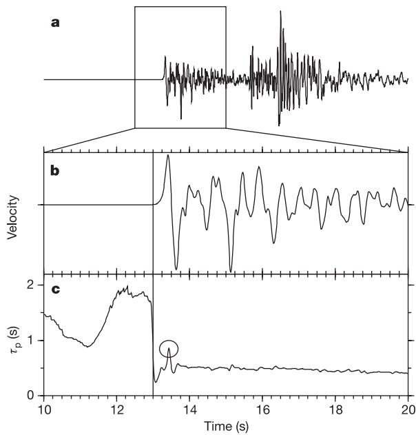
Figure 1 | Example waveform and \tau_p^{\max} calculation for a M 4.6 earthquake in southern California recorded at station GSC, 74 km from the epicentre.
