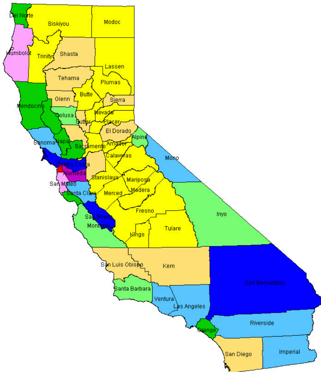
Figure 21. Annual, per-capita building damage economic loss by county, based on the USGS-CGS 2002 PSHA maps, weighted average soil, and liquefaction effect ($).
