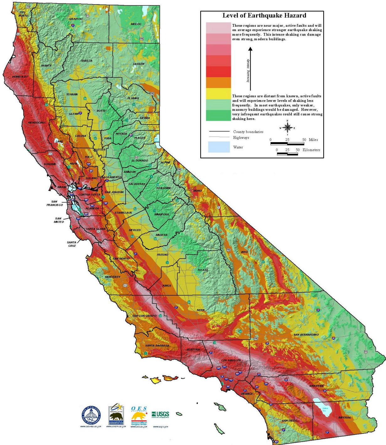
Figure 19 – Earthquake shaking hazard expressed in terms of 1-second spectral acceleration with 10% Probability of Exceedance in 50 Years. Values calculated by CGS from the USGS/CGS seismic shaking model (Frankel, et al., 2002) considering amplification in near surface soils as shown by Wills, et al. (2000) using the amplification factors recommended by the Building Seismic Safety Council (FEMA, 1994, 1997).
