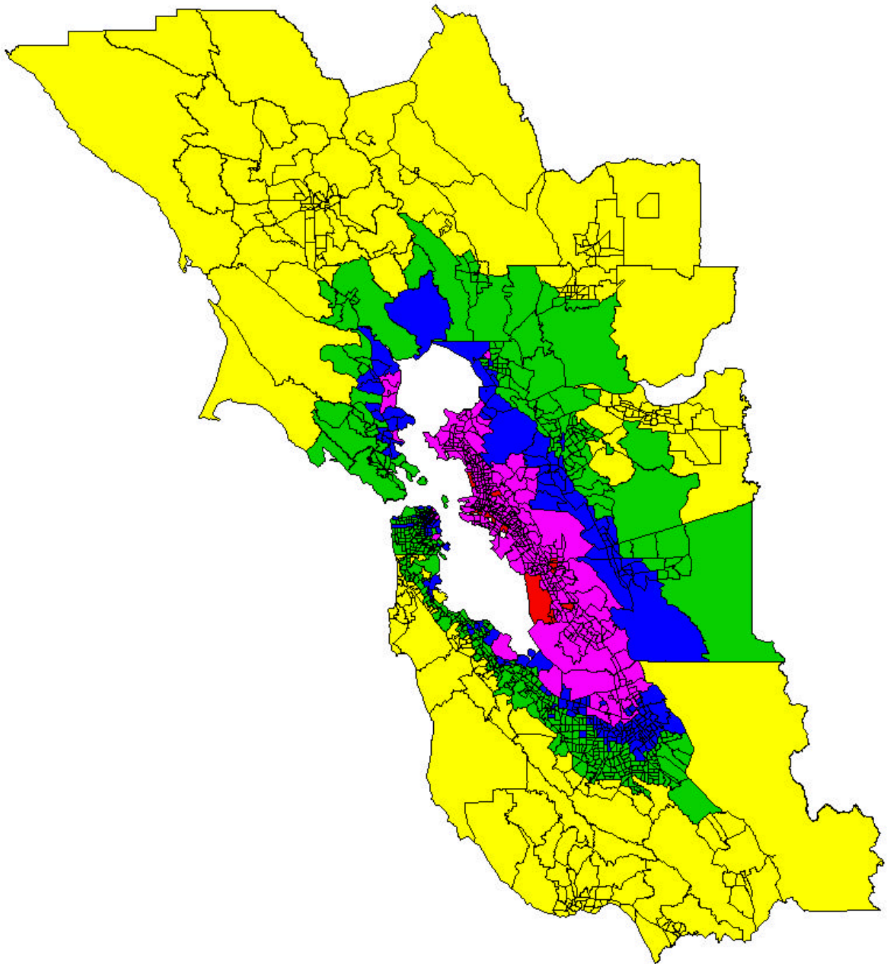
Figure 6. Estimated building damage economic loss as percentage of building replacement value by census tract for southern plus northern Hayward M6.9 scenario earthquake (in parentheses are the numbers of census tracts).
