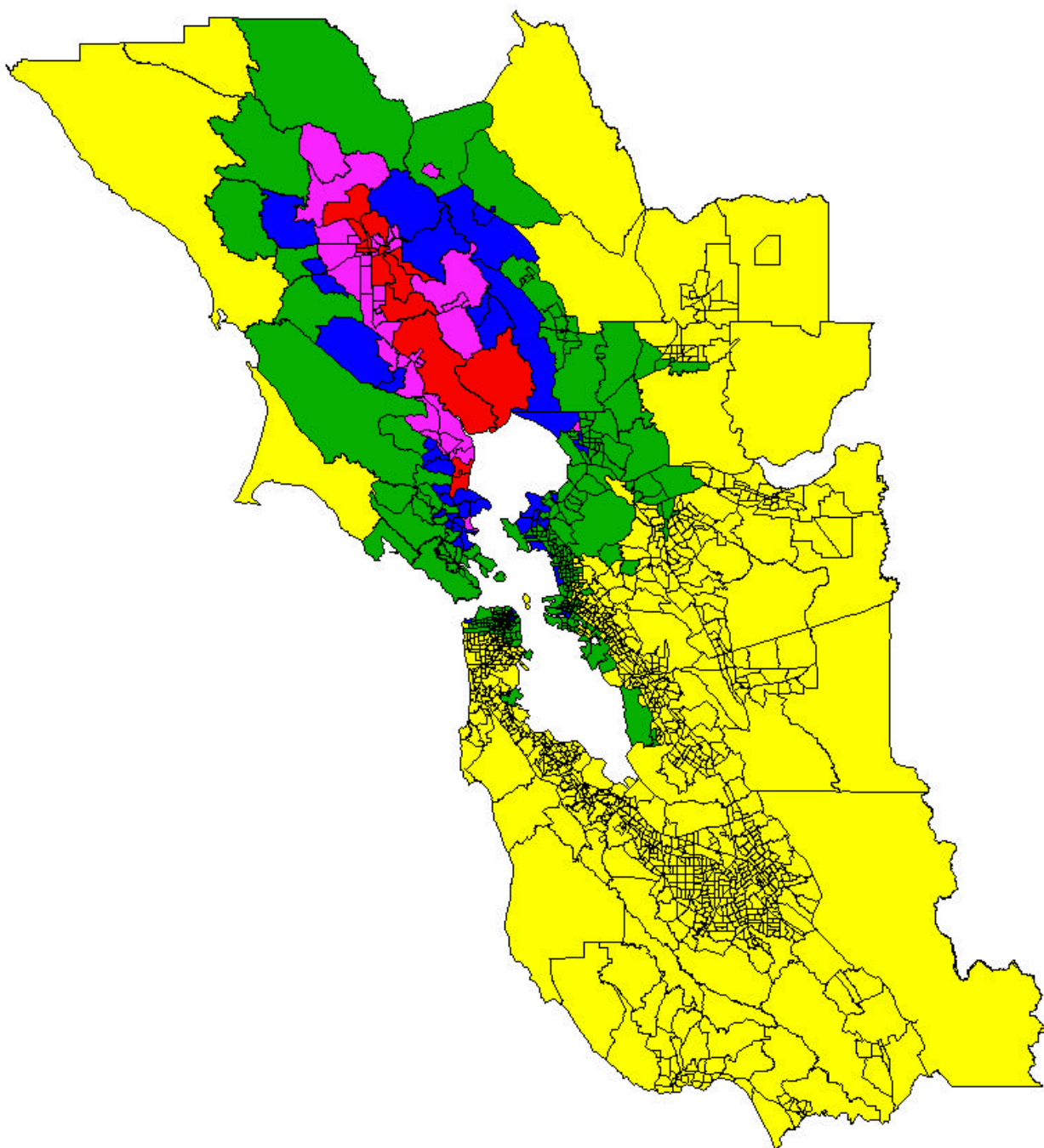
Figure 9. Estimated building damage economic loss as percentage of building replacement value by census tract for Rodgers Creek M7.0 scenario earthquake (in parentheses are the numbers of census tracts).
