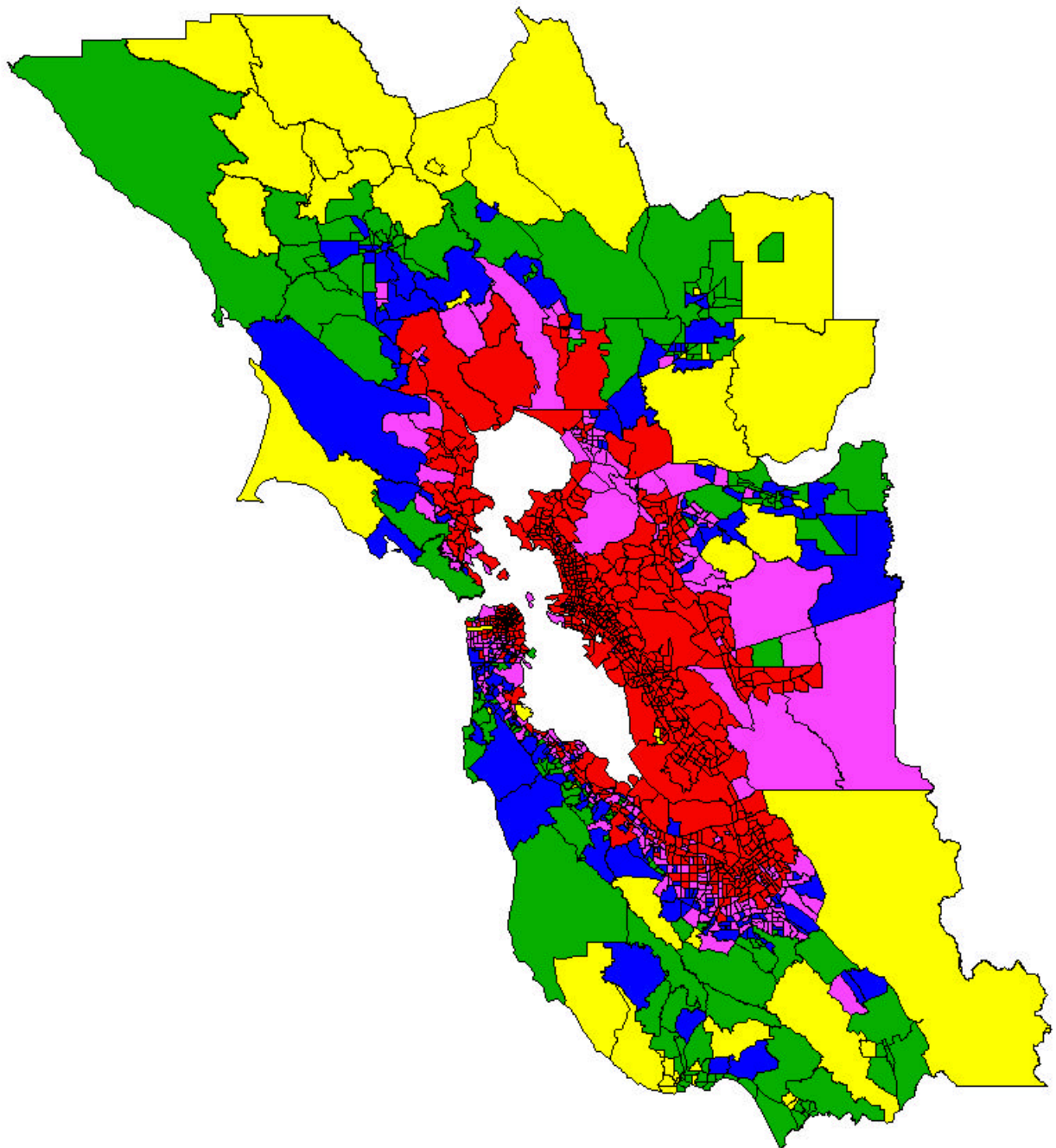
Figure 5. Estimated building damage economic loss by census tract ($1,000) for southern plus northern Hayward M6.9 scenario earthquake (in parentheses are the numbers of census tracts).
