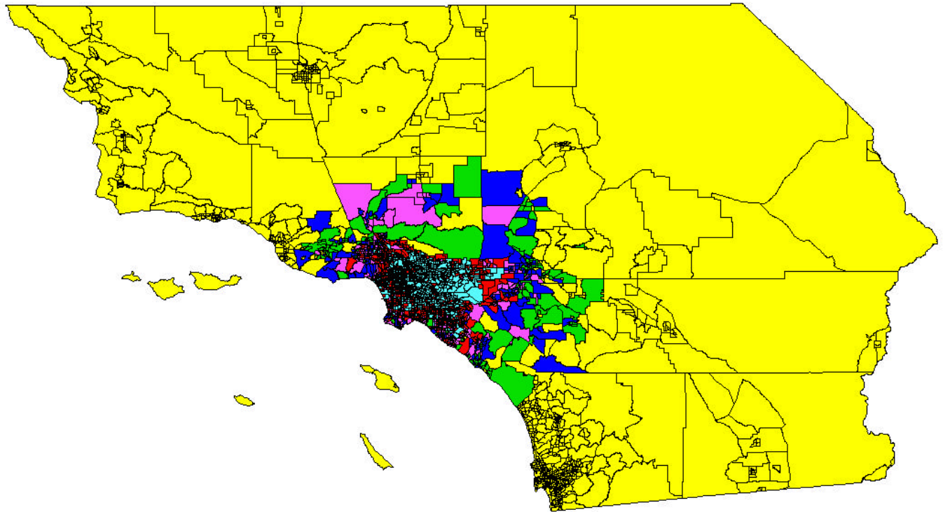
Figure 11. Estimated building damage economic loss by census tract ($1,000) for Puente-Hills M7.1 scenario earthquake (in parentheses are the numbers of census tracts).
