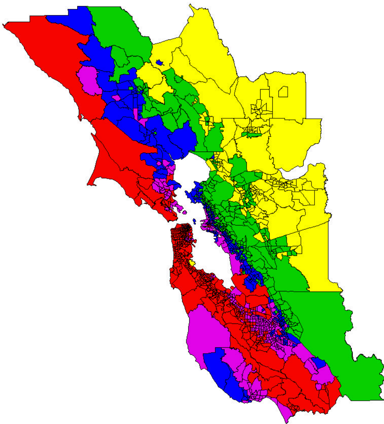
Figure 3. Estimated building damage economic loss as percentage of building replacement value by census tract for a repeat of the 1906 M7.9 San Francisco earthquake (in parentheses are the numbers of census tracts).
